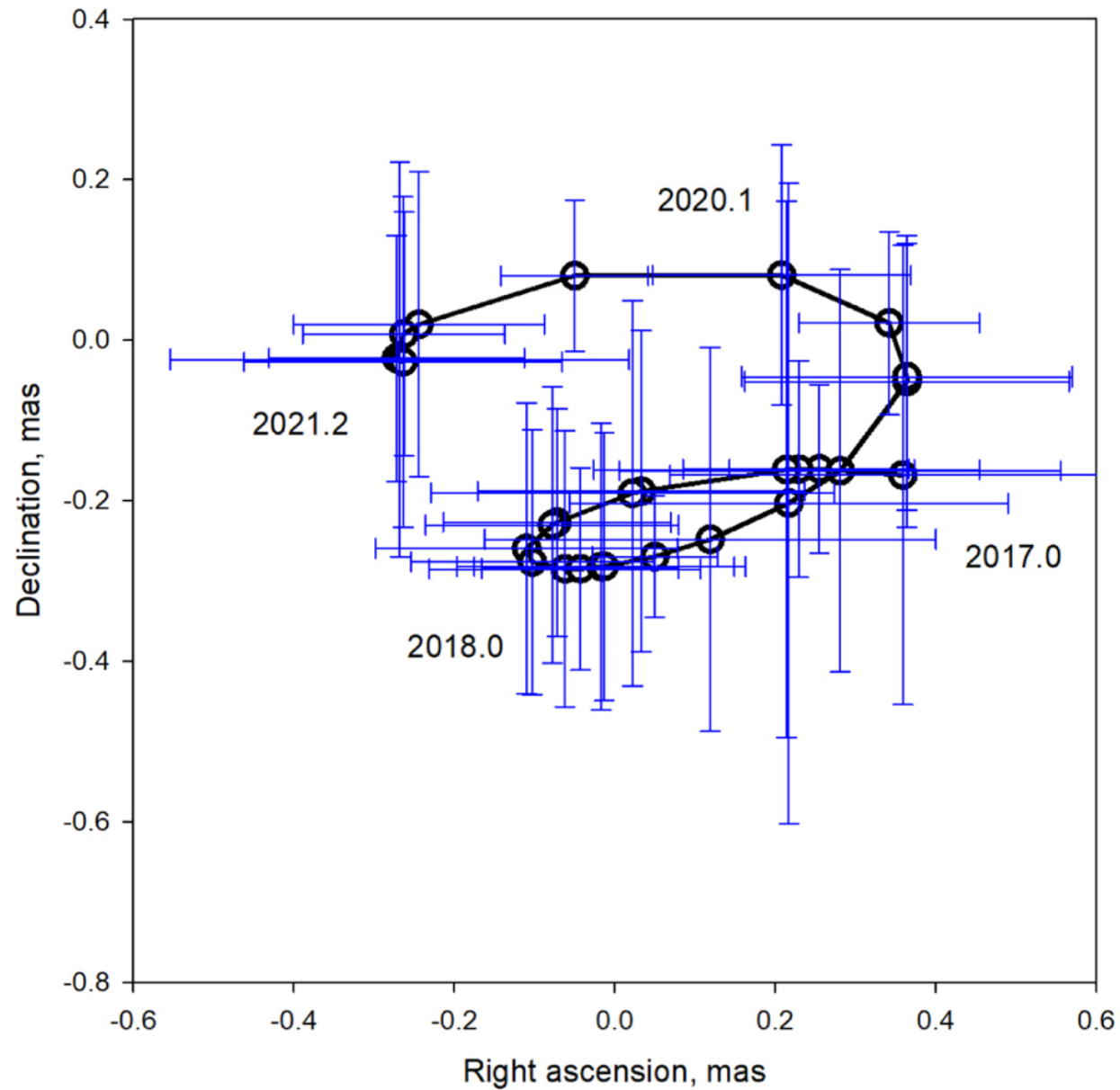
Figure 8. from Oleg Titov et al 2023 Astron. J. 165 doi:10.3847/1538-3881/aca964 https://dx.doi.org/10.3847/1538-3881/aca964 © 2023. The Author(s). Published by the American Astronomical Society.
