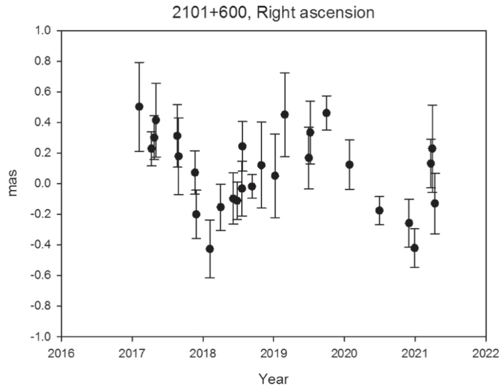
Figure 7. from Oleg Titov et al 2023 Astron. J. 165 doi:10.3847/1538-3881/aca964 https://dx.doi.org/10.3847/1538-3881/aca964 © 2023. The Author(s). Published by the American Astronomical Society.
