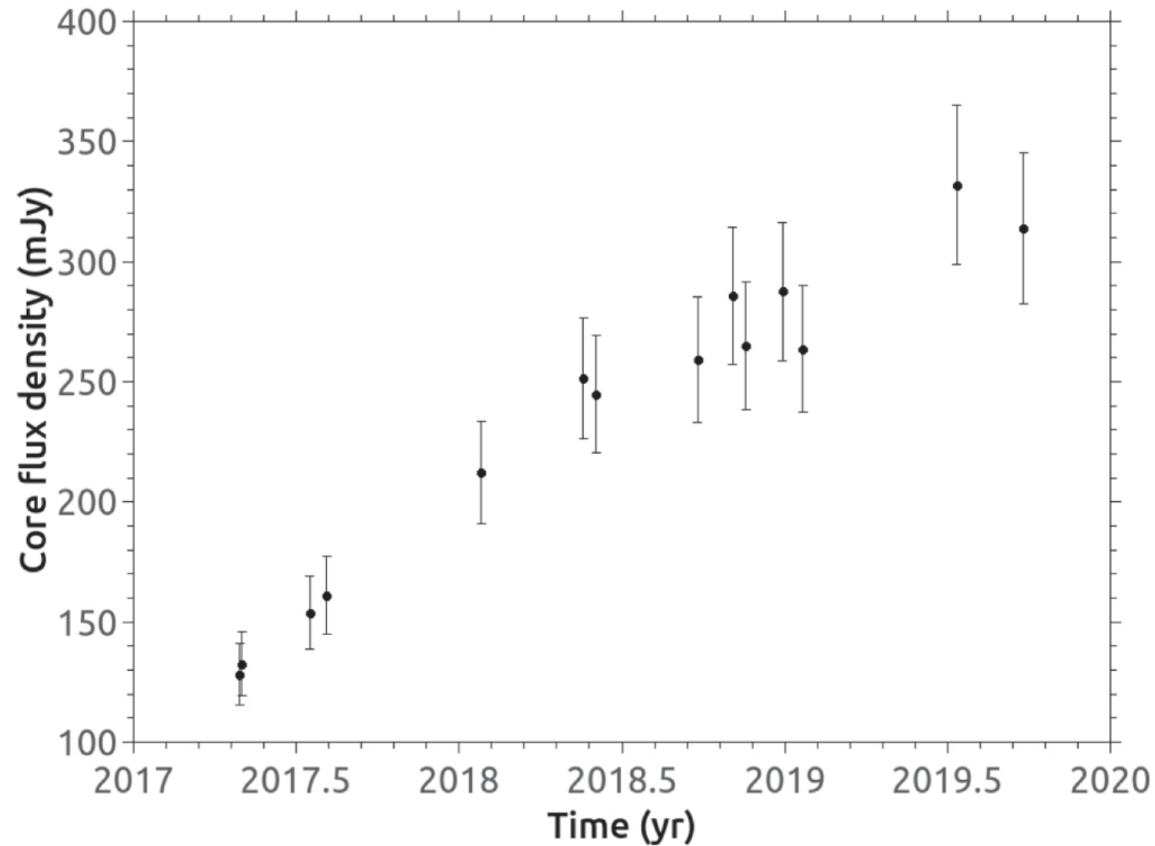
Figure 6. from Oleg Titov et al 2023 Astron. J. 165 doi:10.3847/1538-3881/aca964 https://dx.doi.org/10.3847/1538-3881/aca964 © 2023. The Author(s). Published by the American Astronomical Society.
