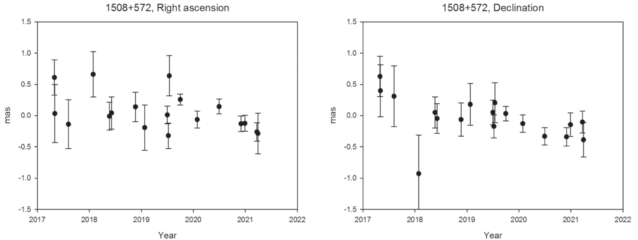
Figure 4. from Oleg Titov et al 2023 Astron. J. 165 doi:10.3847/1538-3881/aca964 https://dx.doi.org/10.3847/1538-3881/aca964 © 2023. The Author(s). Published by the American Astronomical Society.
