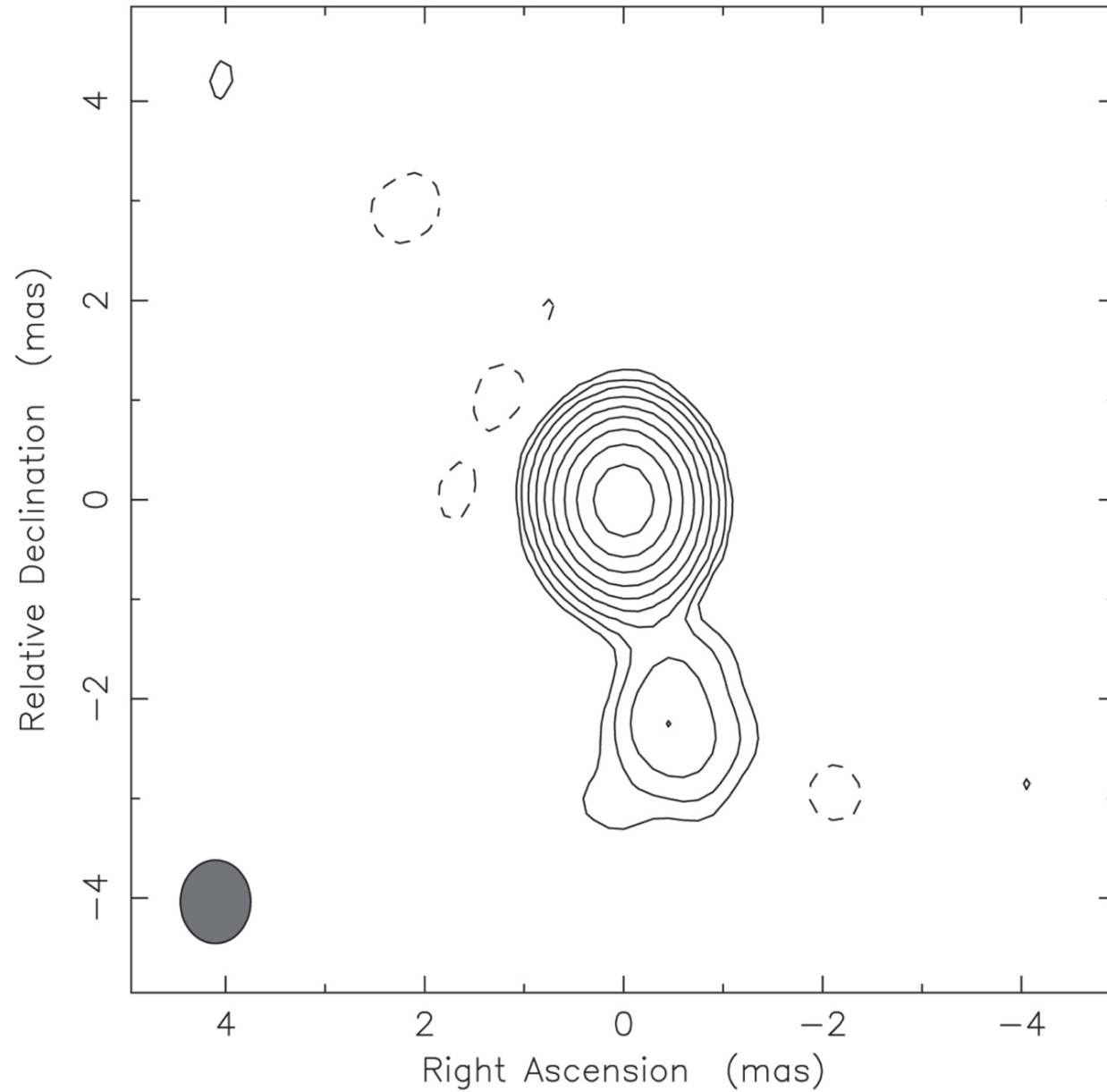
Figure 3. from Oleg Titov et al 2023 Astron. J. 165 doi:10.3847/1538-3881/aca964 https://dx.doi.org/10.3847/1538-3881/aca964 © 2023. The Author(s). Published by the American Astronomical Society.
