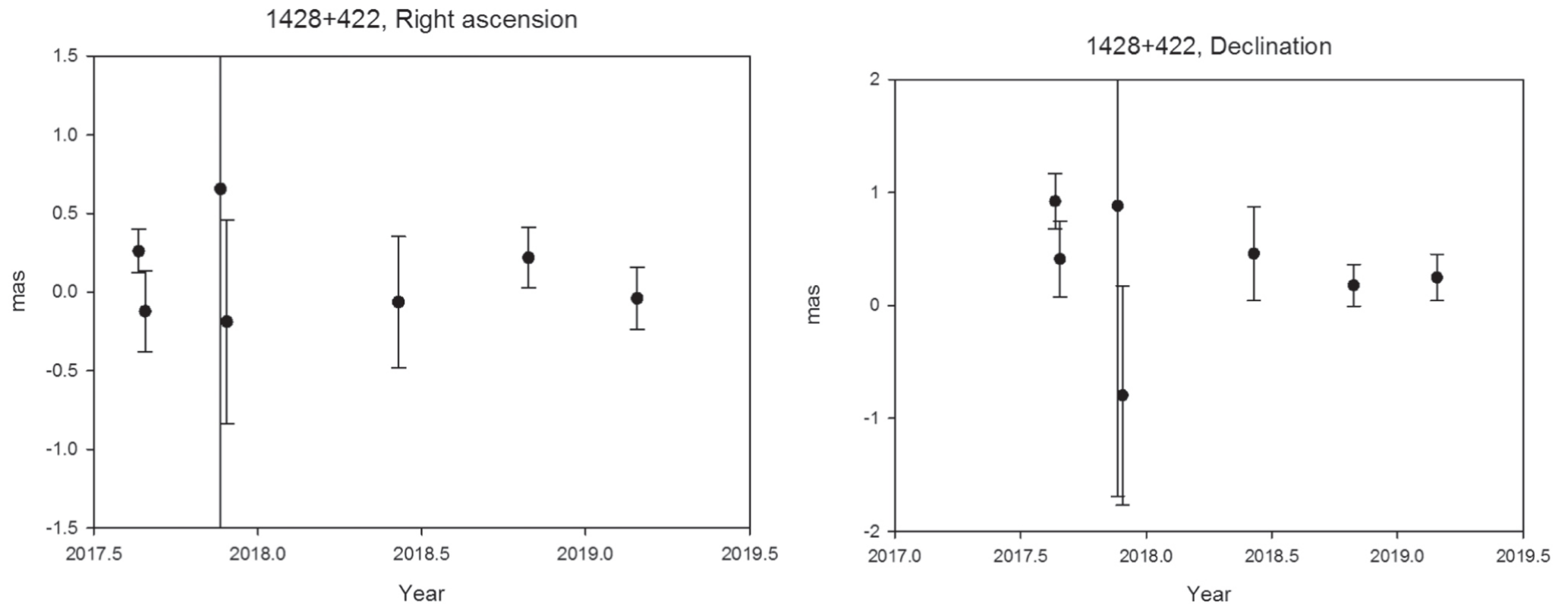
Figure 2. from Oleg Titov et al 2023 Astron. J. 165 doi:10.3847/1538-3881/aca964 https://dx.doi.org/10.3847/1538-3881/aca964 © 2023. The Author(s). Published by the American Astronomical Society.
