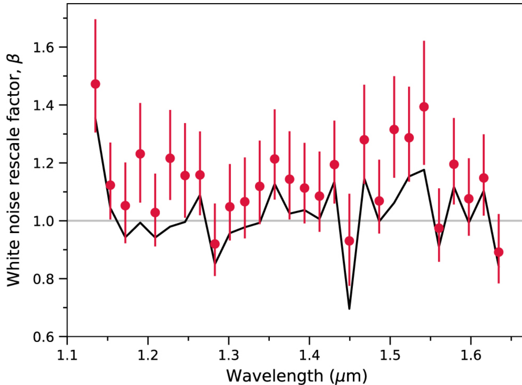
Figure 4. from Thomas Mikal-Evans et al 2023 Astron. J. 165 doi:10.3847/1538-3881/aca90b https://dx.doi.org/10.3847/1538-3881/aca90b © 2023. The Author(s). Published by the American Astronomical Society.
