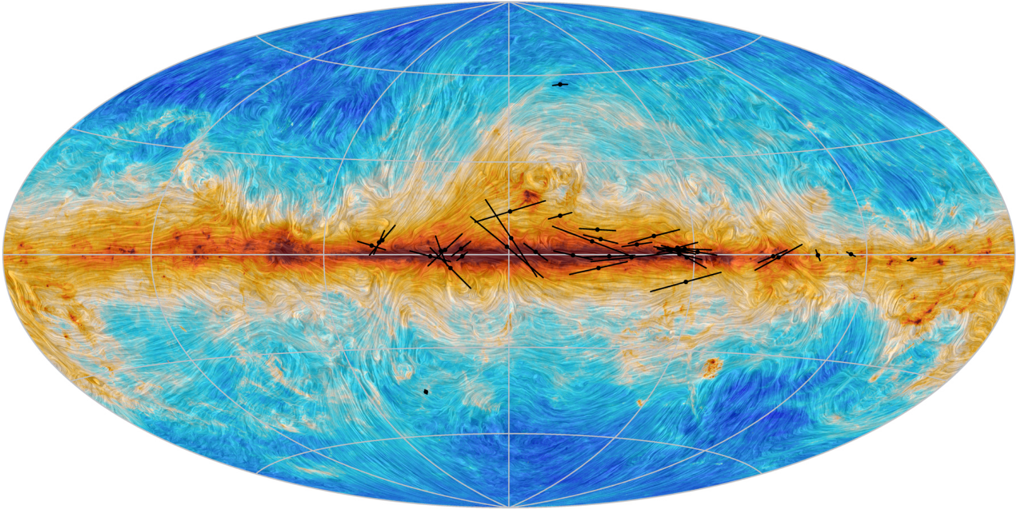
Figure 8. from M. J. F. Versteeg et al 2023 Astron. J. 165 doi:10.3847/1538-3881/aca8fd https://dx.doi.org/10.3847/1538-3881/aca8fd © 2023. The Author(s). Published by the American Astronomical Society.
