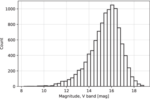
Figure 6. from M. J. F. Versteeg et al 2023 Astron. J. 165 doi:10.3847/1538-3881/aca8fd https://dx.doi.org/10.3847/1538-3881/aca8fd © 2023. The Author(s). Published by the American Astronomical Society.
