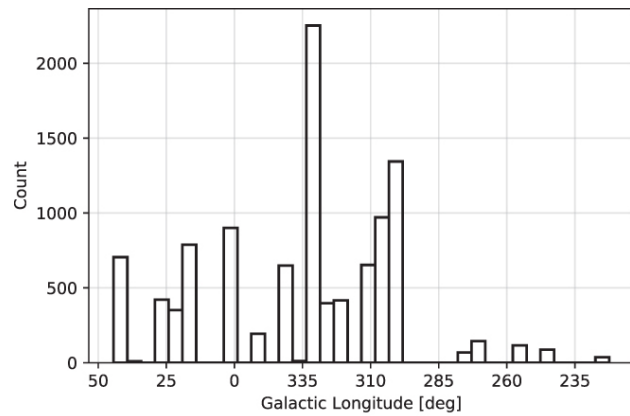
Figure 5. from M. J. F. Versteeg et al 2023 Astron. J. 165 doi:10.3847/1538-3881/aca8fd https://dx.doi.org/10.3847/1538-3881/aca8fd © 2023. The Author(s). Published by the American Astronomical Society.
