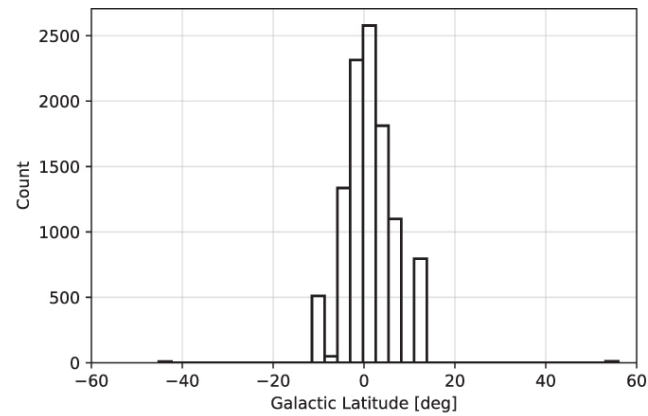
Figure 5. from M. J. F. Versteeg et al 2023 Astron. J. 165 doi:10.3847/1538-3881/aca8fd https://dx.doi.org/10.3847/1538-3881/aca8fd © 2023. The Author(s). Published by the American Astronomical Society.
