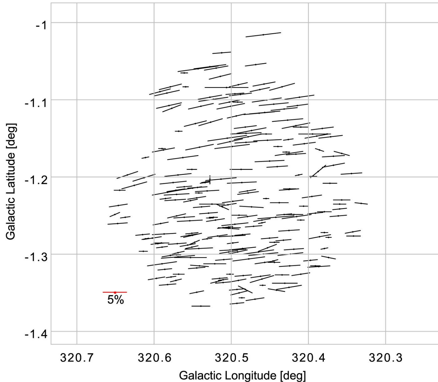
Figure 3. from M. J. F. Versteeg et al 2023 Astron. J. 165 doi:10.3847/1538-3881/aca8fd https://dx.doi.org/10.3847/1538-3881/aca8fd © 2023. The Author(s). Published by the American Astronomical Society.
