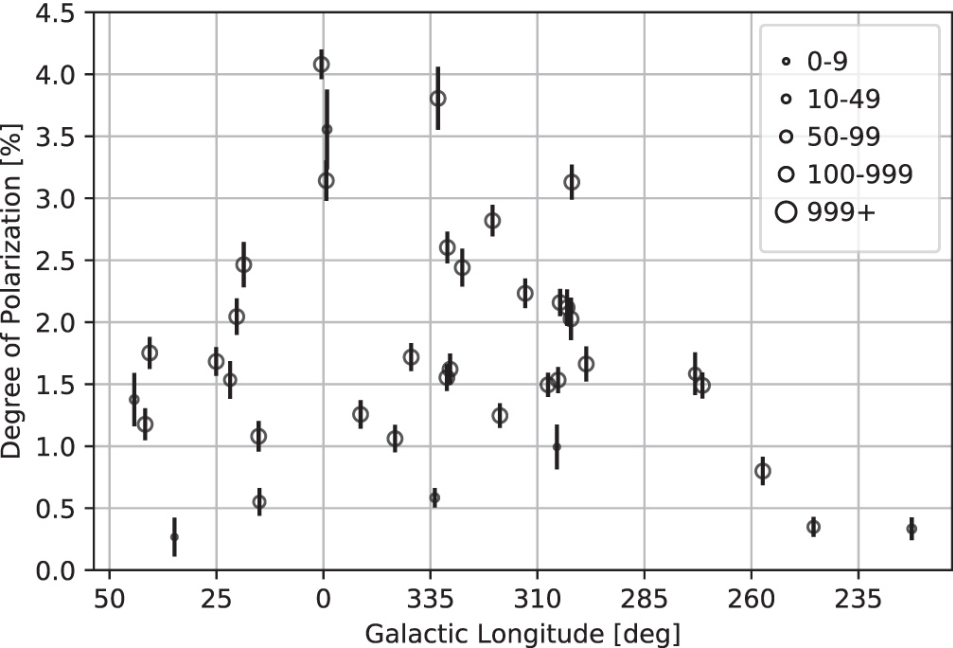
Figure 11. from M. J. F. Versteeg et al 2023 Astron. J. 165 doi:10.3847/1538-3881/aca8fd https://dx.doi.org/10.3847/1538-3881/aca8fd © 2023. The Author(s). Published by the American Astronomical Society.
