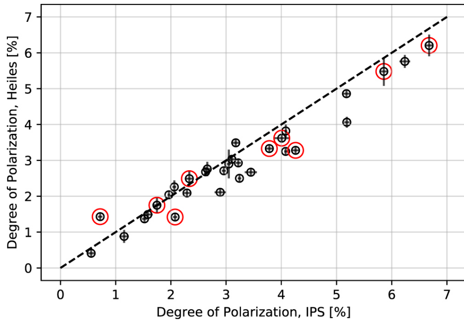
Figure 1. from M. J. F. Versteeg et al 2023 Astron. J. 165 doi:10.3847/1538-3881/aca8fd https://dx.doi.org/10.3847/1538-3881/aca8fd © 2023. The Author(s). Published by the American Astronomical Society.
