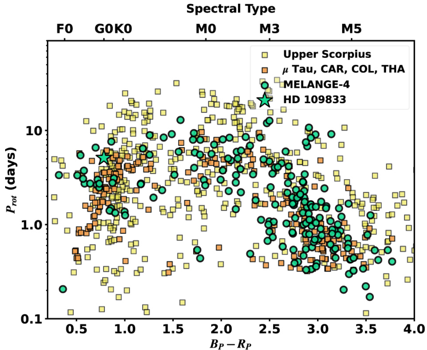
Figure 4. from Mackenna L. Wood et al 2023 Astron. J. 165 doi:10.3847/1538-3881/aca8fc https://dx.doi.org/10.3847/1538-3881/aca8fc © 2023. The Author(s). Published by the American Astronomical Society.
