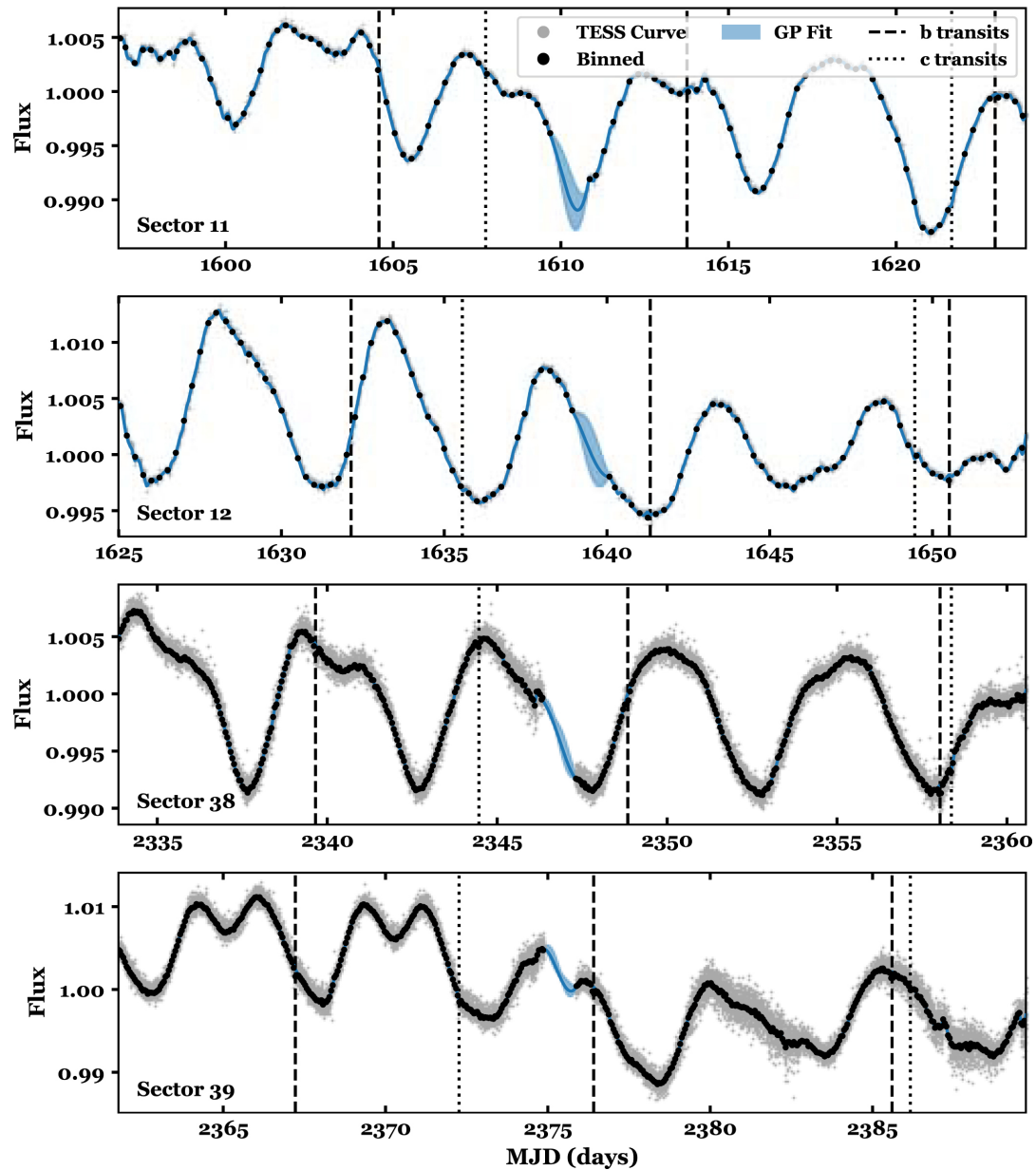
Figure 10. from Mackenna L. Wood et al 2023 Astron. J. 165 doi:10.3847/1538-3881/aca8fc https://dx.doi.org/10.3847/1538-3881/aca8fc © 2023. The Author(s). Published by the American Astronomical Society.
