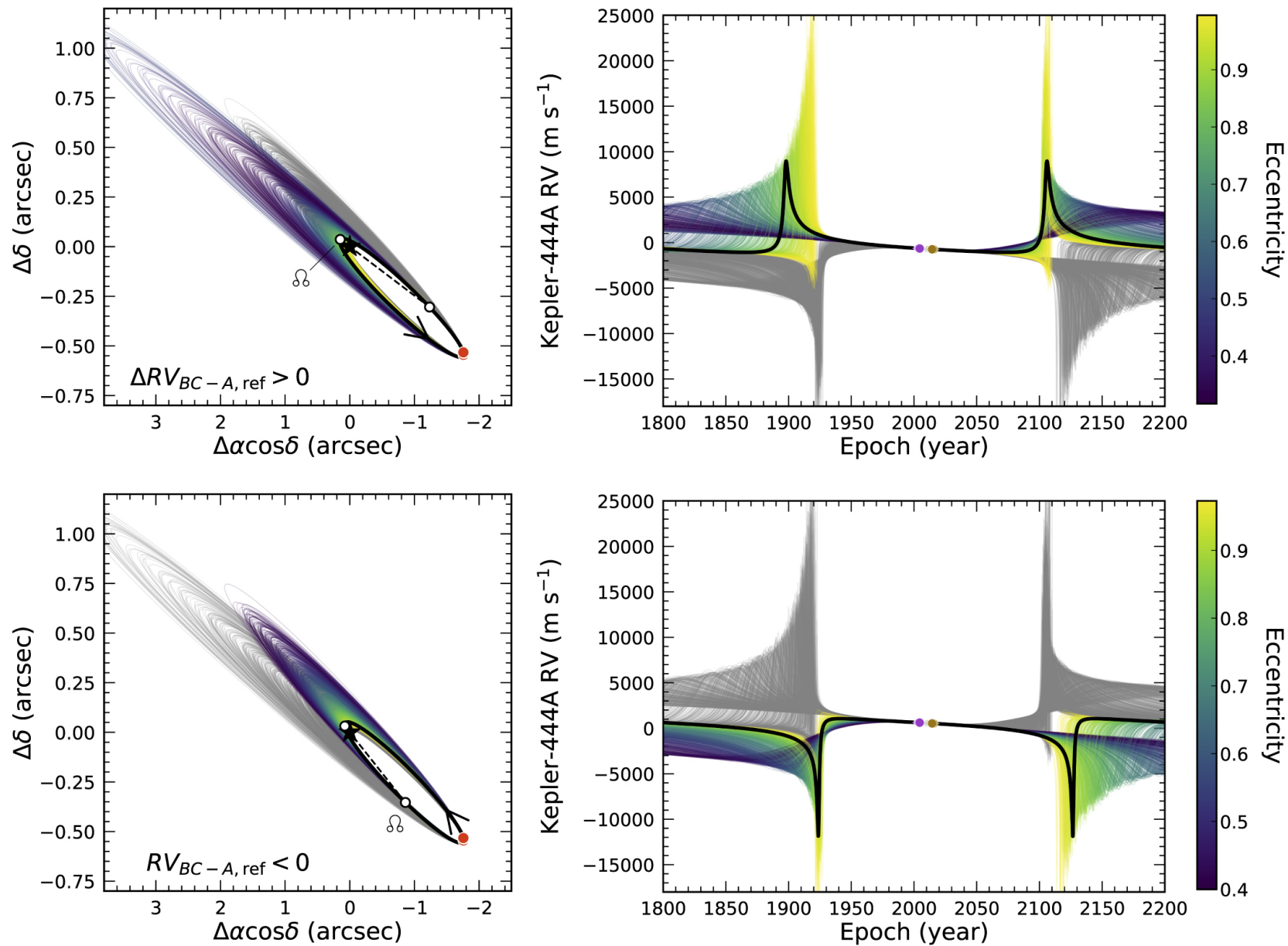
Figure 7. from Zhoujian Zhang et al 2023 Astron. J. 165 doi:10.3847/1538-3881/aca88c https://dx.doi.org/10.3847/1538-3881/aca88c © 2023. The Author(s). Published by the American Astronomical Society.
