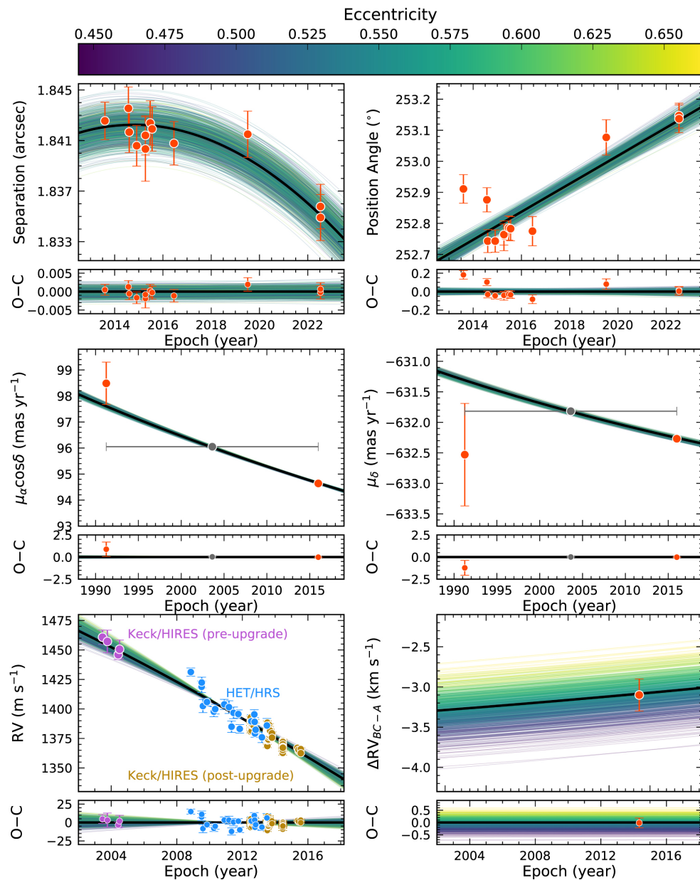
Figure 5. from Zhoujian Zhang et al 2023 Astron. J. 165 doi:10.3847/1538-3881/aca88c https://dx.doi.org/10.3847/1538-3881/aca88c © 2023. The Author(s). Published by the American Astronomical Society.
