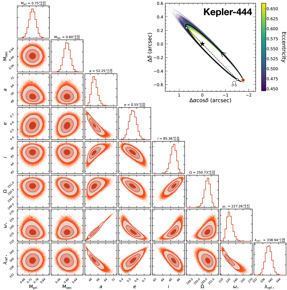
Figure 4. from Zhoujian Zhang et al 2023 Astron. J. 165 doi:10.3847/1538-3881/aca88c https://dx.doi.org/10.3847/1538-3881/aca88c © 2023. The Author(s). Published by the American Astronomical Society.
