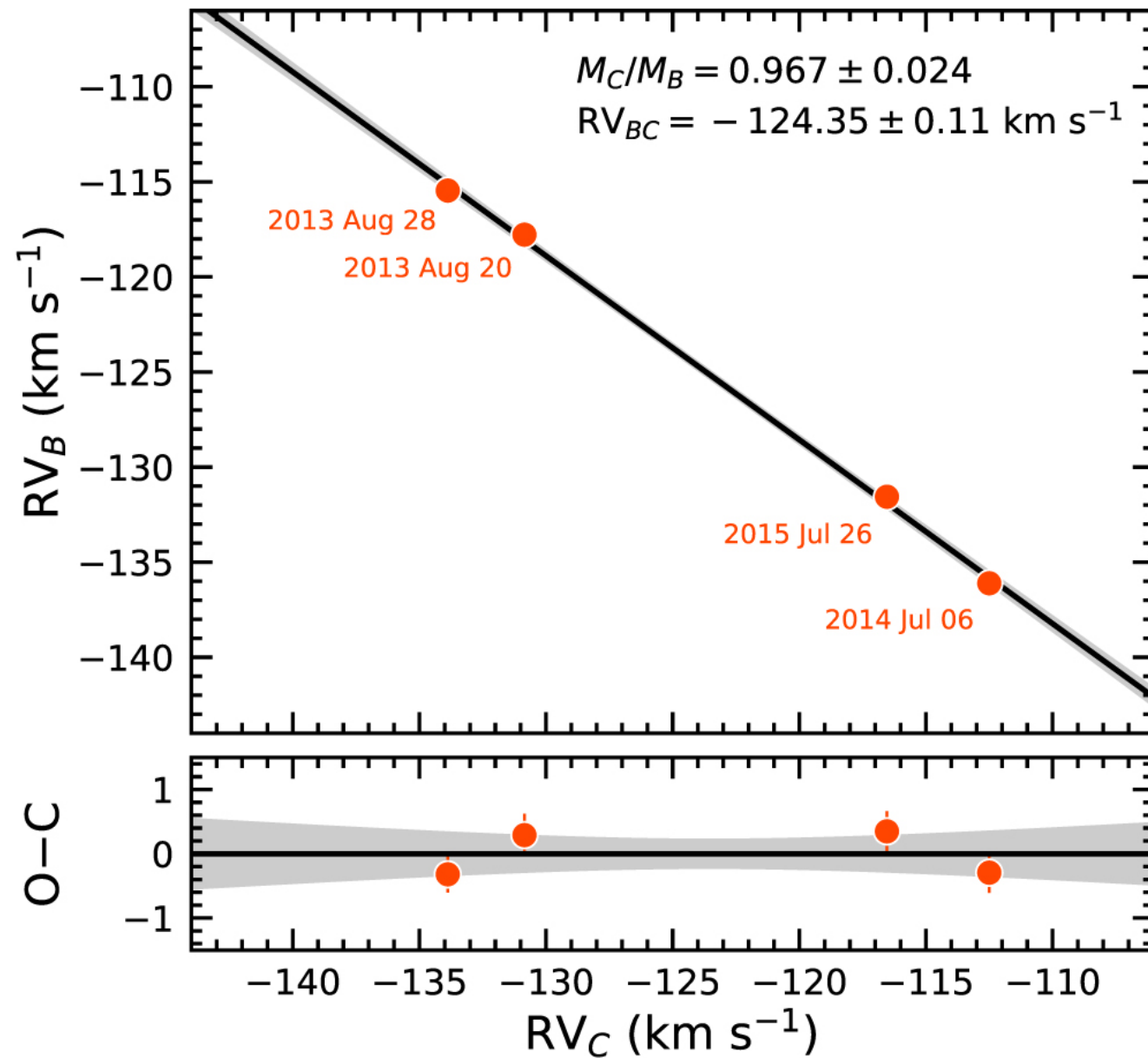
Figure 3. from Zhoujian Zhang et al 2023 Astron. J. 165 doi:10.3847/1538-3881/aca88c https://dx.doi.org/10.3847/1538-3881/aca88c © 2023. The Author(s). Published by the American Astronomical Society.
