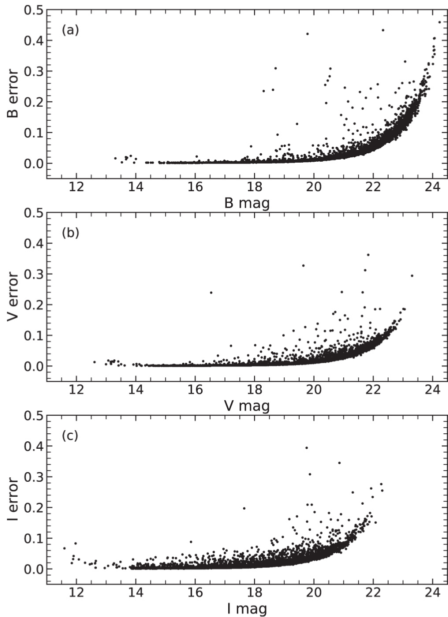
Figure 2. from Hyobin Im et al 2023 Astron. J. 165 doi:10.3847/1538-3881/aca7fb https://dx.doi.org/10.3847/1538-3881/aca7fb © 2023. The Author(s). Published by the American Astronomical Society.
