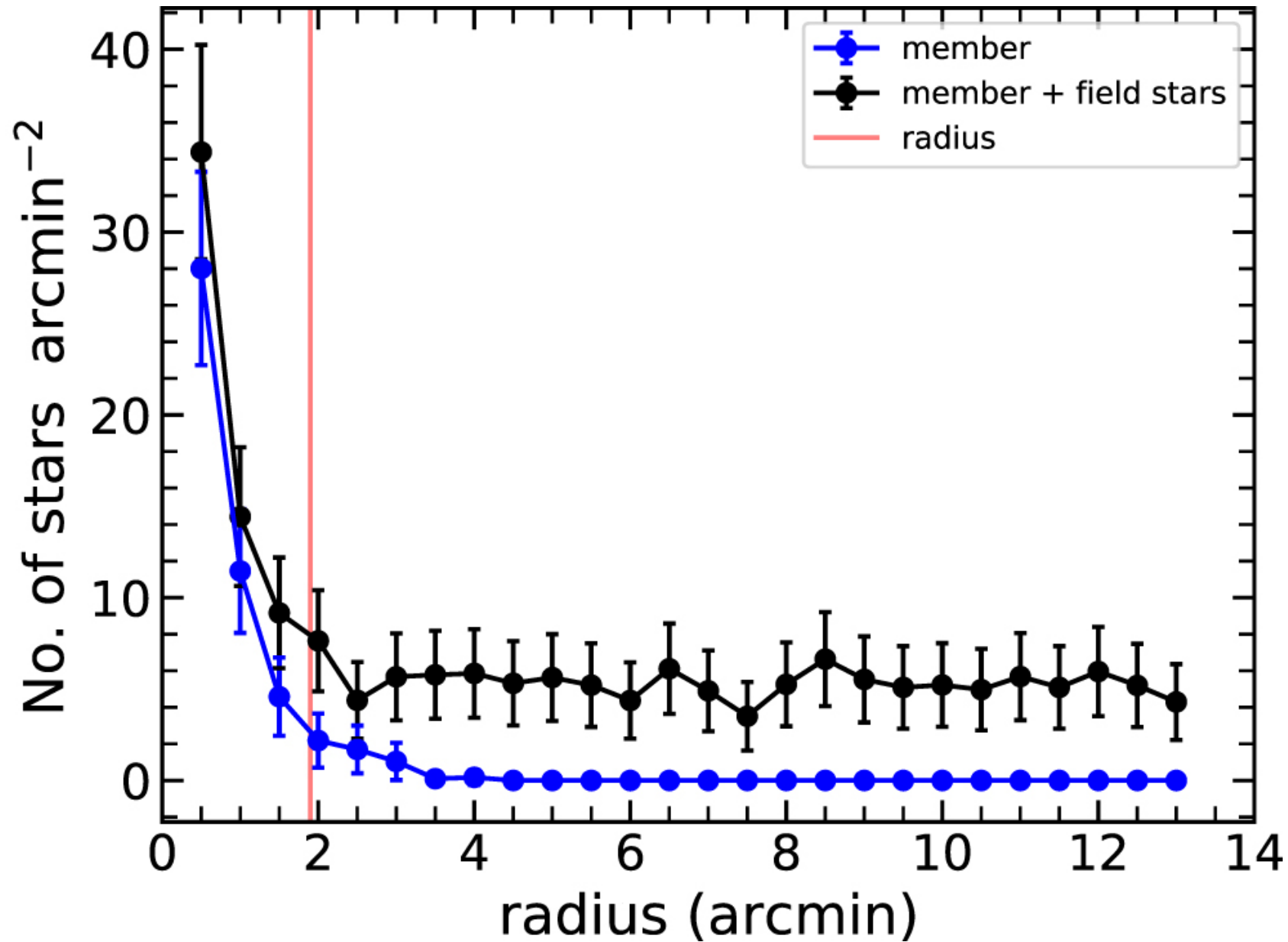
Figure 10. from Hyobin Im et al 2023 Astron. J. 165 doi:10.3847/1538-3881/aca7fb https://dx.doi.org/10.3847/1538-3881/aca7fb © 2023. The Author(s). Published by the American Astronomical Society.
