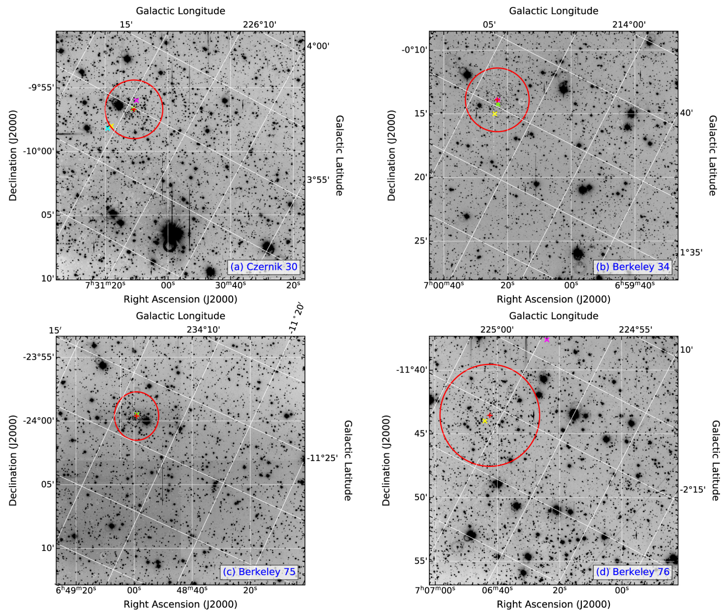
Figure 1. from Hyobin Im et al 2023 Astron. J. 165 doi:10.3847/1538-3881/aca7fb https://dx.doi.org/10.3847/1538-3881/aca7fb © 2023. The Author(s). Published by the American Astronomical Society.
