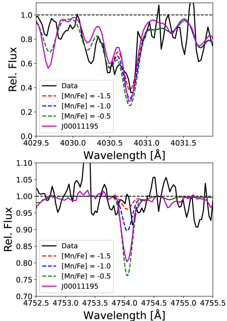
Figure 6. from Anirudh Chiti et al 2023 Astron. J. 165 doi:10.3847/1538-3881/aca416 https://dx.doi.org/10.3847/1538-3881/aca416 © 2023. The Author(s). Published by the American Astronomical Society.
