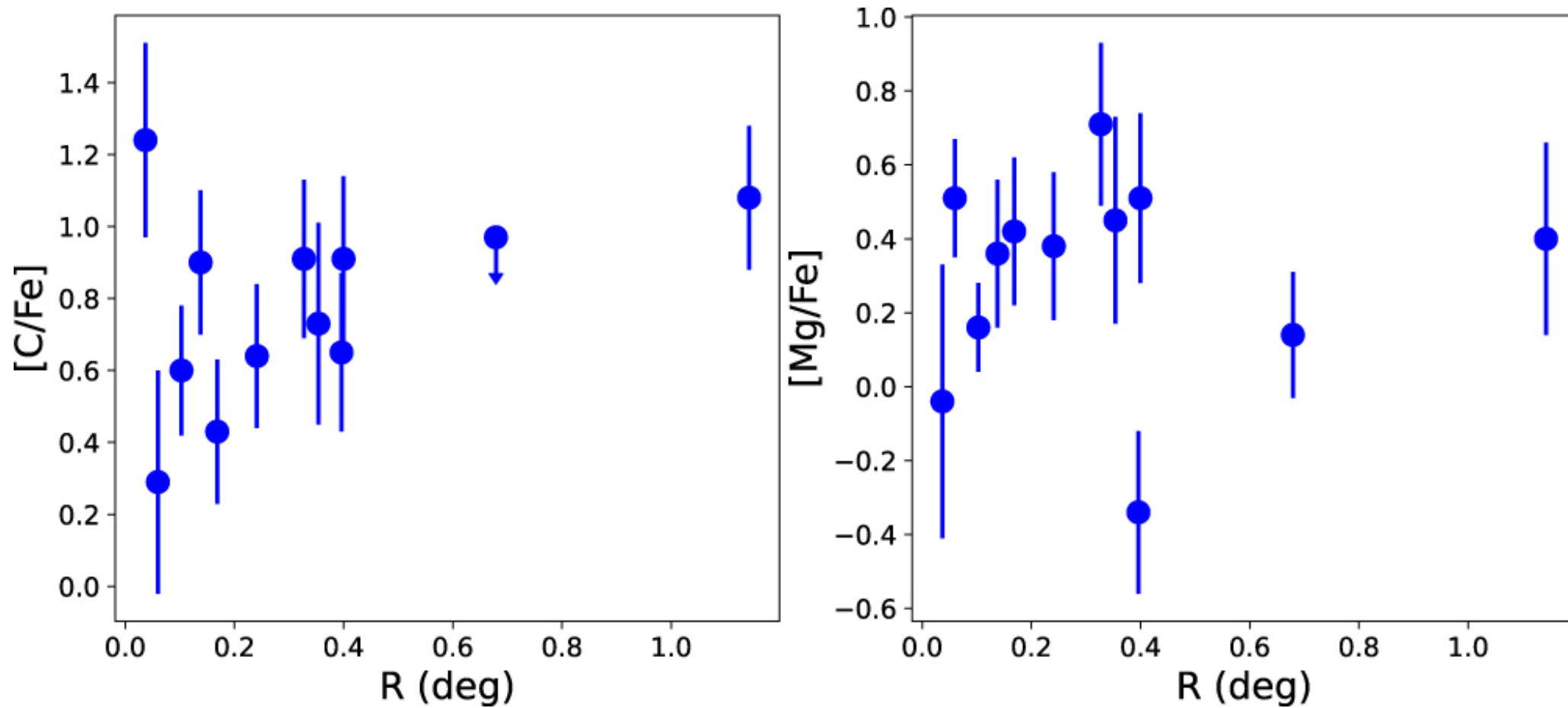
Figure 5. from Anirudh Chiti et al 2023 Astron. J. 165 doi:10.3847/1538-3881/aca416 https://dx.doi.org/10.3847/1538-3881/aca416 © 2023. The Author(s). Published by the American Astronomical Society.
