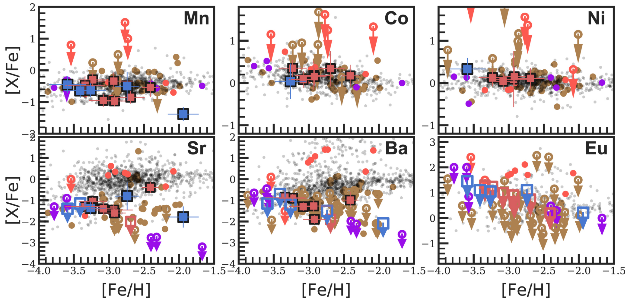
Figure 4. from Anirudh Chiti et al 2023 Astron. J. 165 doi:10.3847/1538-3881/aca416 https://dx.doi.org/10.3847/1538-3881/aca416 © 2023. The Author(s). Published by the American Astronomical Society.
