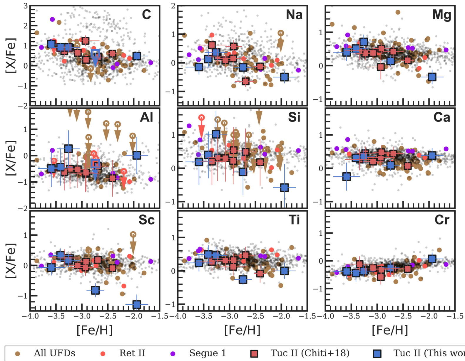
Figure 3. from Anirudh Chiti et al 2023 Astron. J. 165 doi:10.3847/1538-3881/aca416 https://dx.doi.org/10.3847/1538-3881/aca416 © 2023. The Author(s). Published by the American Astronomical Society.
