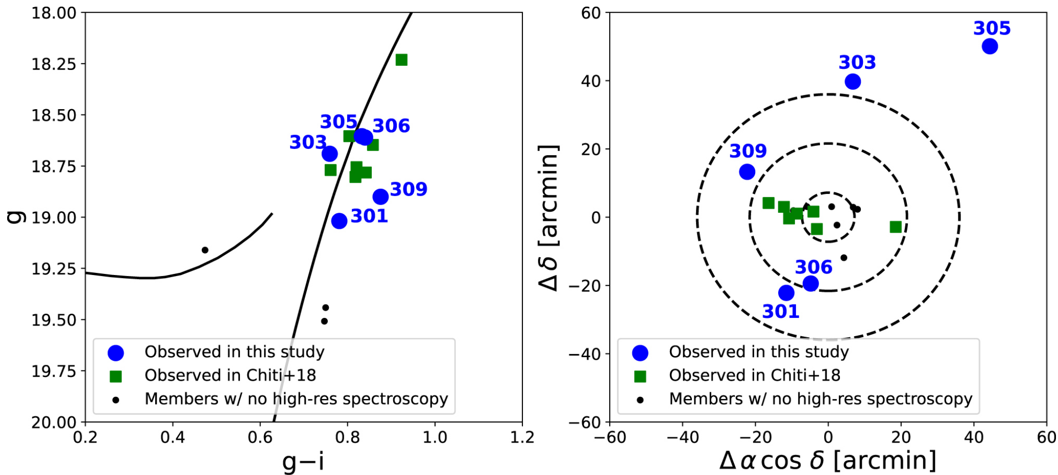
Figure 1. from Anirudh Chiti et al 2023 Astron. J. 165 doi:10.3847/1538-3881/aca416 https://dx.doi.org/10.3847/1538-3881/aca416 © 2023. The Author(s). Published by the American Astronomical Society.
