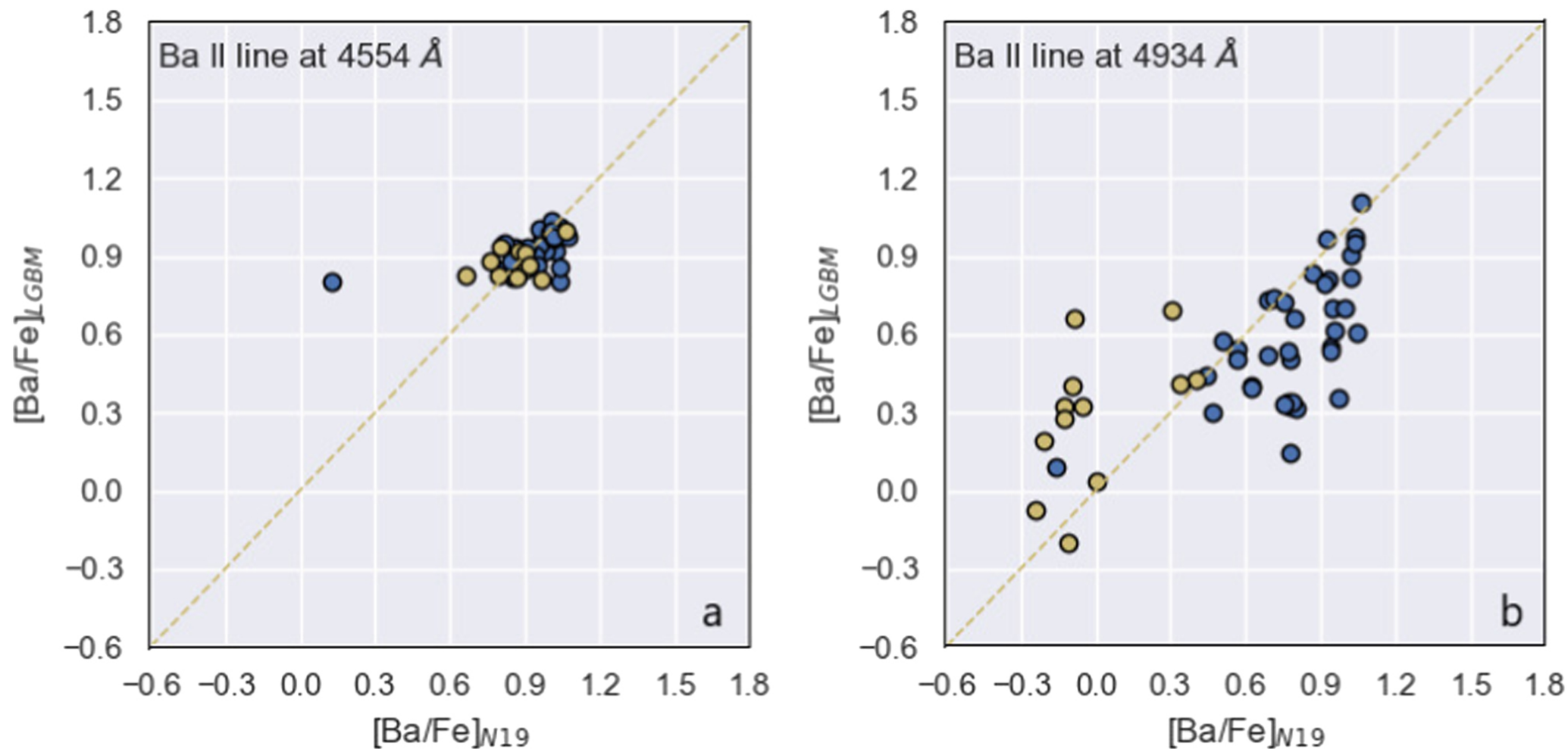
Figure 5. from Fengyue Guo et al 2023 Astron. J. 165 doi:10.3847/1538-3881/aca323 https://dx.doi.org/10.3847/1538-3881/aca323 © 2023. The Author(s). Published by the American Astronomical Society.
