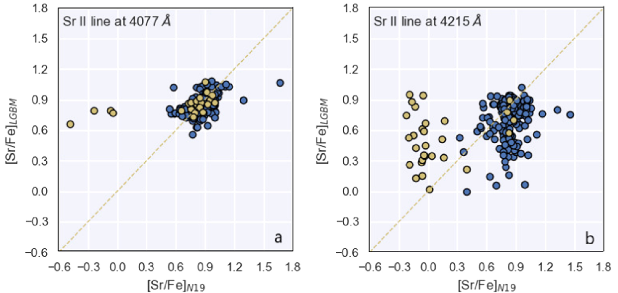
Figure 4. from Fengyue Guo et al 2023 Astron. J. 165 doi:10.3847/1538-3881/aca323 https://dx.doi.org/10.3847/1538-3881/aca323 © 2023. The Author(s). Published by the American Astronomical Society.
