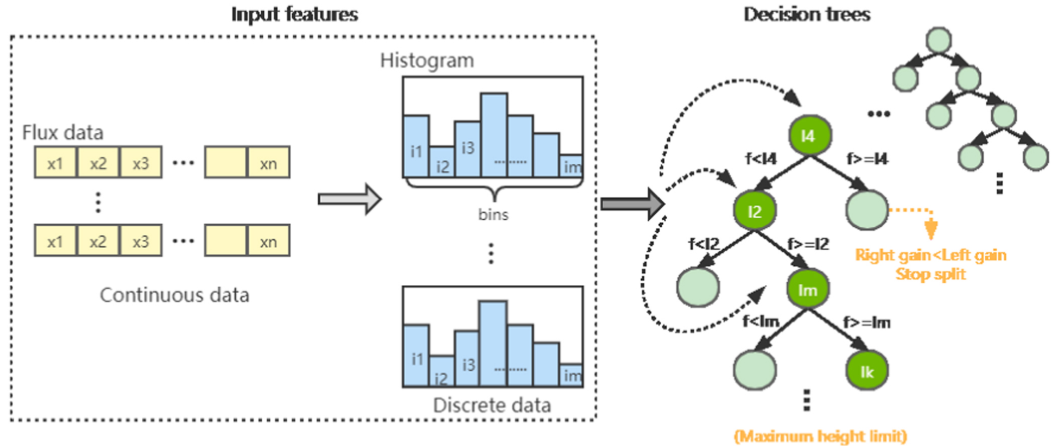
Figure 2. from Fengyue Guo et al 2023 Astron. J. 165 doi:10.3847/1538-3881/aca323 https://dx.doi.org/10.3847/1538-3881/aca323 © 2023. The Author(s). Published by the American Astronomical Society.
