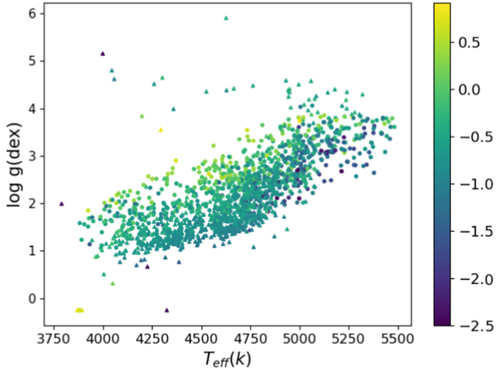
Figure 1. from Fengyue Guo et al 2023 Astron. J. 165 doi:10.3847/1538-3881/aca323 https://dx.doi.org/10.3847/1538-3881/aca323 © 2023. The Author(s). Published by the American Astronomical Society.
