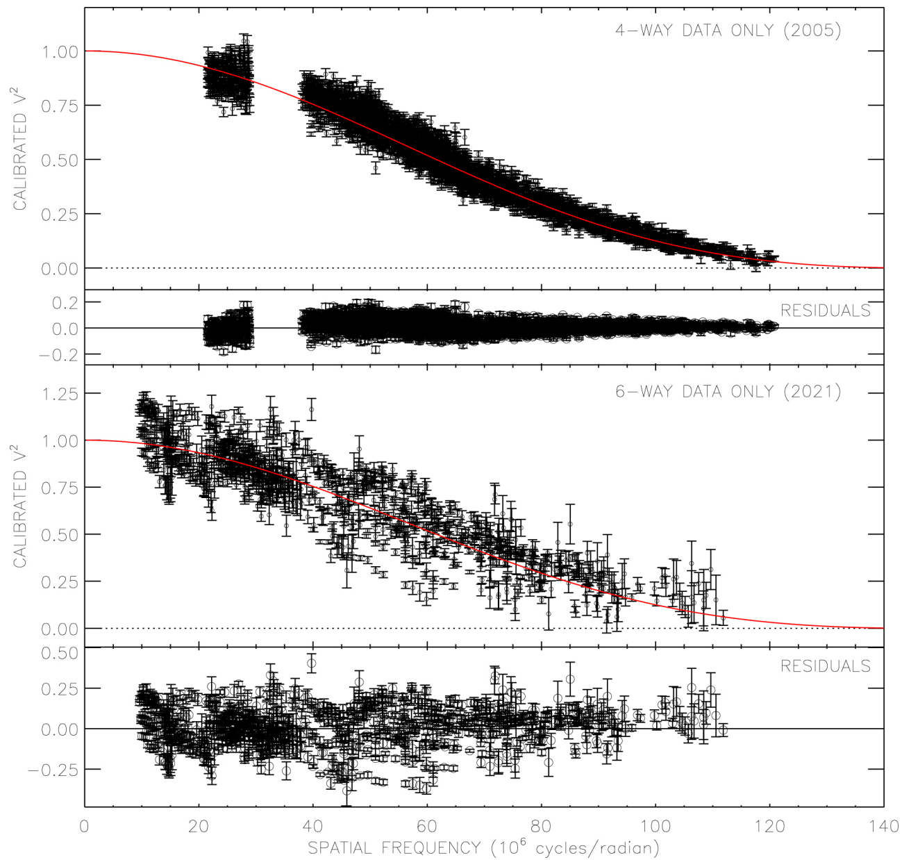
Figure 4. from Ellyn K. Baines et al 2023 Astron. J. 165 doi:10.3847/1538-3881/aca277 https://dx.doi.org/10.3847/1538-3881/aca277 © 2023. The Author(s). Published by the American Astronomical Society.
