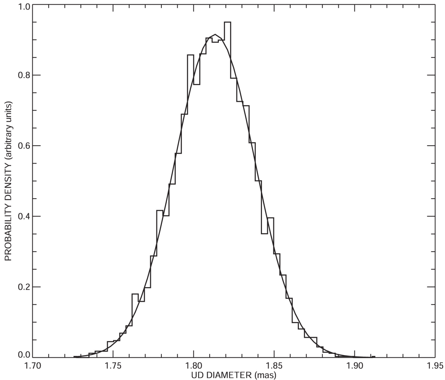
Figure 3. from Ellyn K. Baines et al 2023 Astron. J. 165 doi:10.3847/1538-3881/aca277 https://dx.doi.org/10.3847/1538-3881/aca277 © 2023. The Author(s). Published by the American Astronomical Society.
