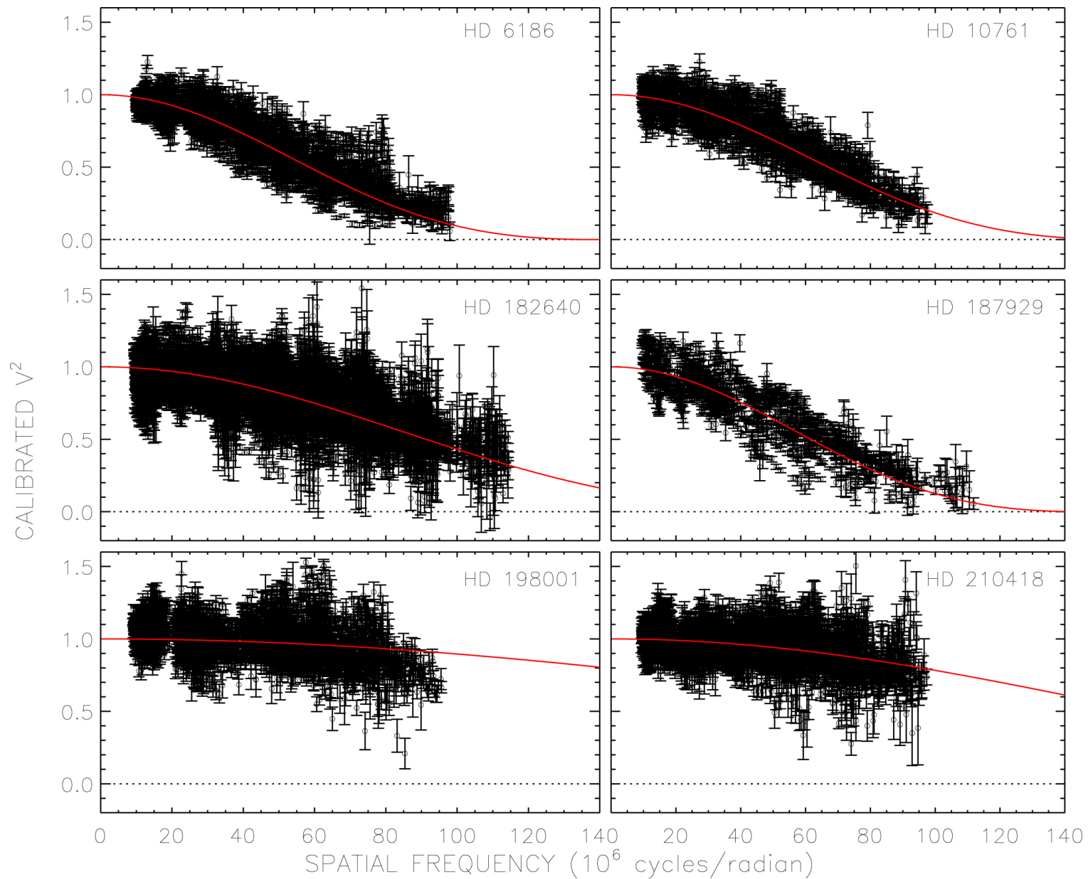
Figure 2. from Ellyn K. Baines et al 2023 Astron. J. 165 doi:10.3847/1538-3881/aca277 https://dx.doi.org/10.3847/1538-3881/aca277 © 2023. The Author(s). Published by the American Astronomical Society.
