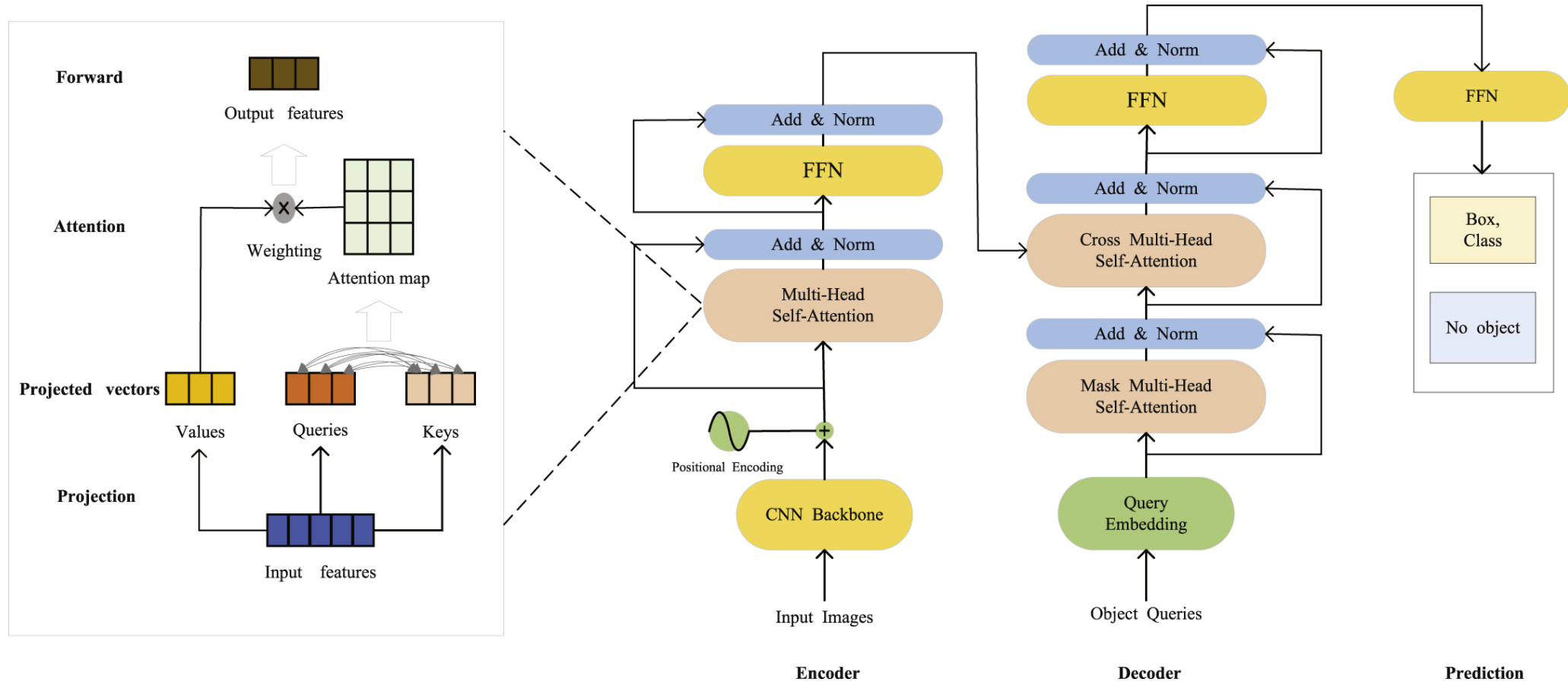
Figure 5. from Peng Jia et al 2023 Astron. J. 165 doi:10.3847/1538-3881/aca1c2 https://dx.doi.org/10.3847/1538-3881/aca1c2 © 2022. The Author(s). Published by the American Astronomical Society.
