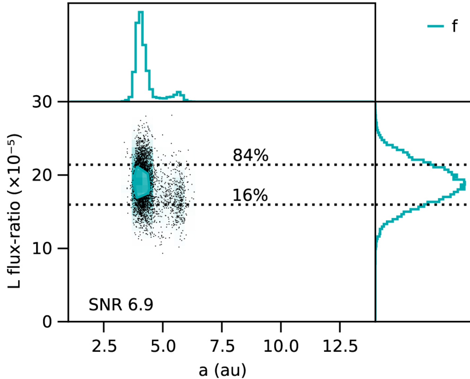
Figure 8. from William Thompson et al 2023 Astron. J. 165 doi:10.3847/1538-3881/aca1af https://dx.doi.org/10.3847/1538-3881/aca1af © 2022. The Author(s). Published by the American Astronomical Society.
