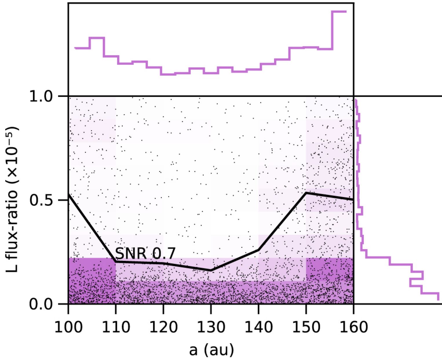
Figure 7. from William Thompson et al 2023 Astron. J. 165 doi:10.3847/1538-3881/aca1af https://dx.doi.org/10.3847/1538-3881/aca1af © 2022. The Author(s). Published by the American Astronomical Society.
