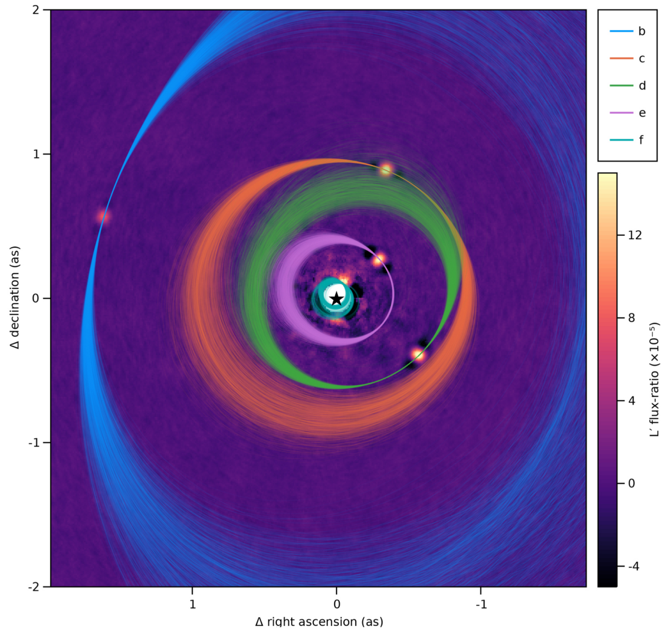
Figure 4. from William Thompson et al 2023 Astron. J. 165 doi:10.3847/1538-3881/aca1af https://dx.doi.org/10.3847/1538-3881/aca1af © 2022. The Author(s). Published by the American Astronomical Society.
