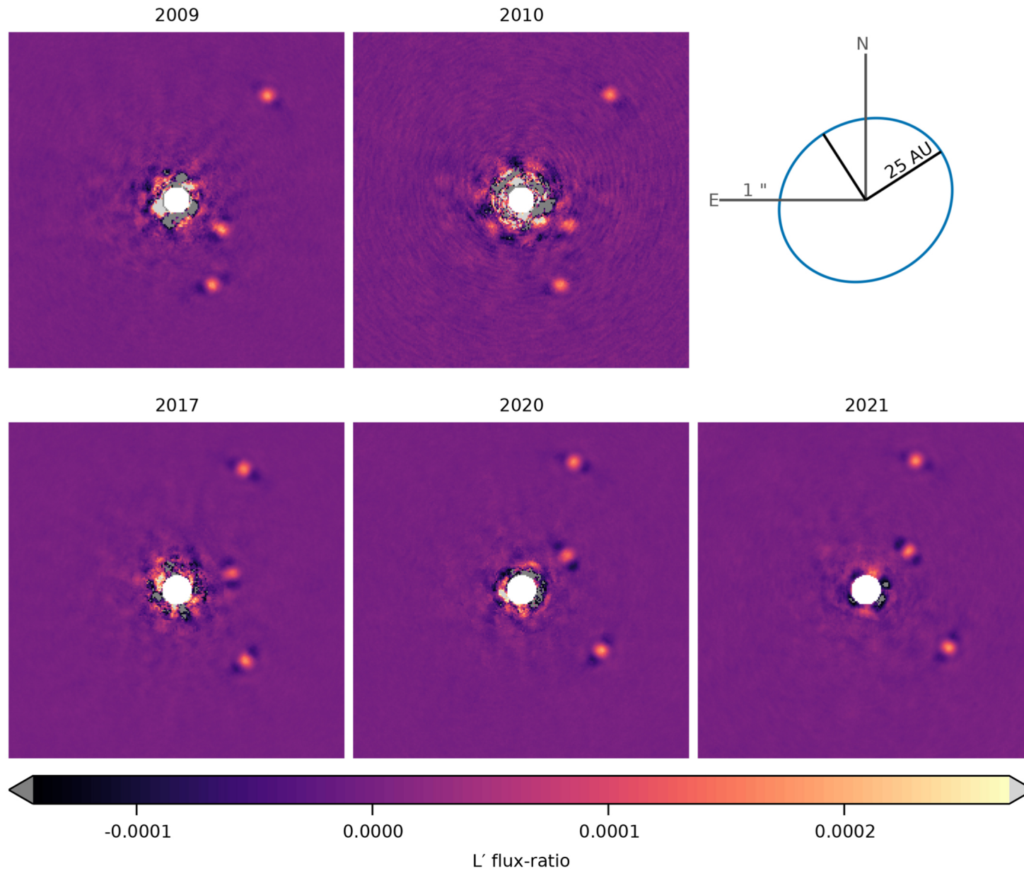
Figure 2. from William Thompson et al 2023 Astron. J. 165 doi:10.3847/1538-3881/aca1af https://dx.doi.org/10.3847/1538-3881/aca1af © 2022. The Author(s). Published by the American Astronomical Society.
