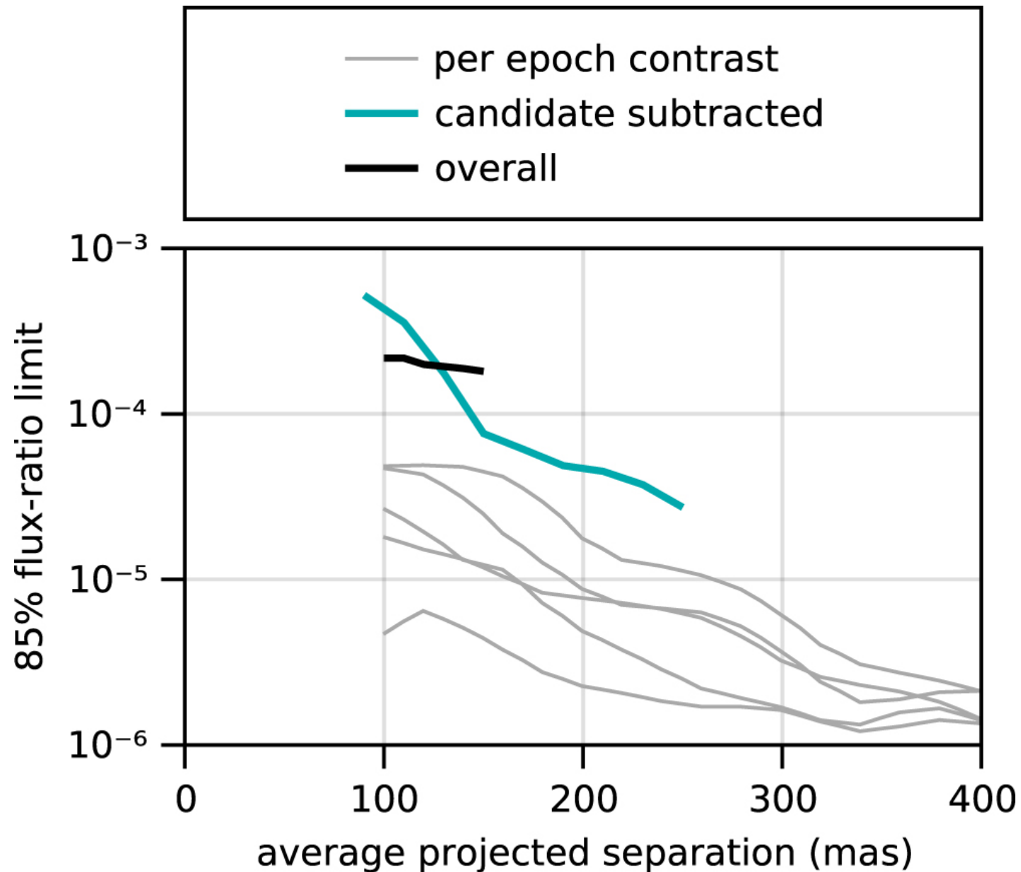
Figure 15. from William Thompson et al 2023 Astron. J. 165 doi:10.3847/1538-3881/aca1af https://dx.doi.org/10.3847/1538-3881/aca1af © 2022. The Author(s). Published by the American Astronomical Society.
