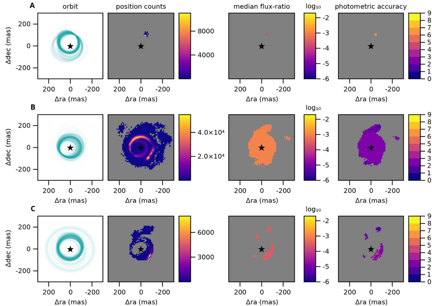
Figure 10. from William Thompson et al 2023 Astron. J. 165 doi:10.3847/1538-3881/aca1af https://dx.doi.org/10.3847/1538-3881/aca1af © 2022. The Author(s). Published by the American Astronomical Society.
