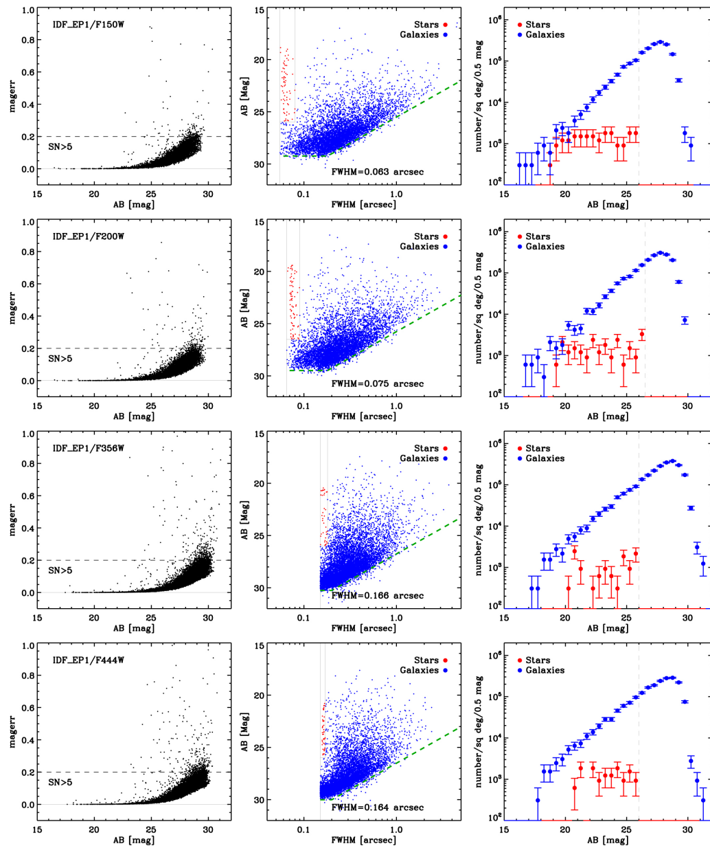
Figure 8. from Rogier A. Windhorst et al 2023 Astron. J. 165 doi:10.3847/1538-3881/aca163 https://dx.doi.org/10.3847/1538-3881/aca163 © 2022. The Author(s). Published by the American Astronomical Society.
