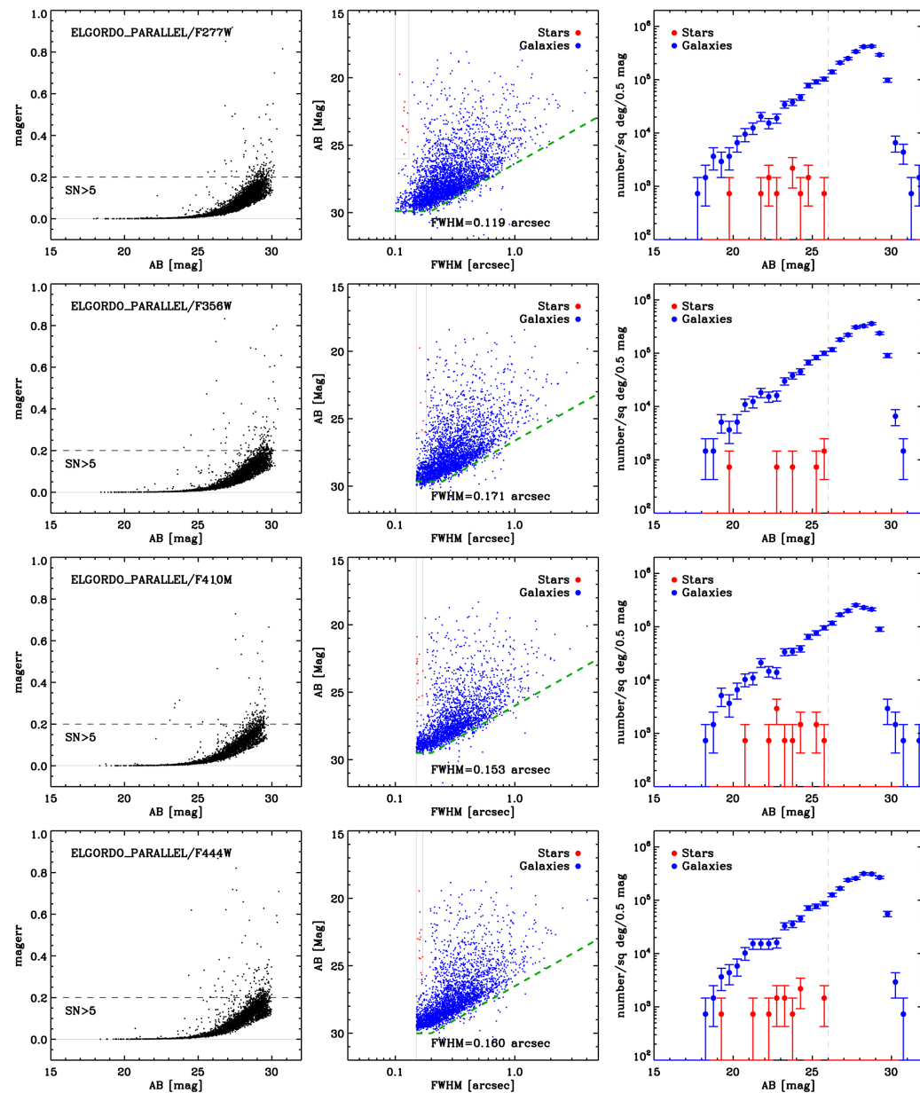
Figure 7. from Rogier A. Windhorst et al 2023 Astron. J. 165 doi:10.3847/1538-3881/aca163 https://dx.doi.org/10.3847/1538-3881/aca163 © 2022. The Author(s). Published by the American Astronomical Society.
