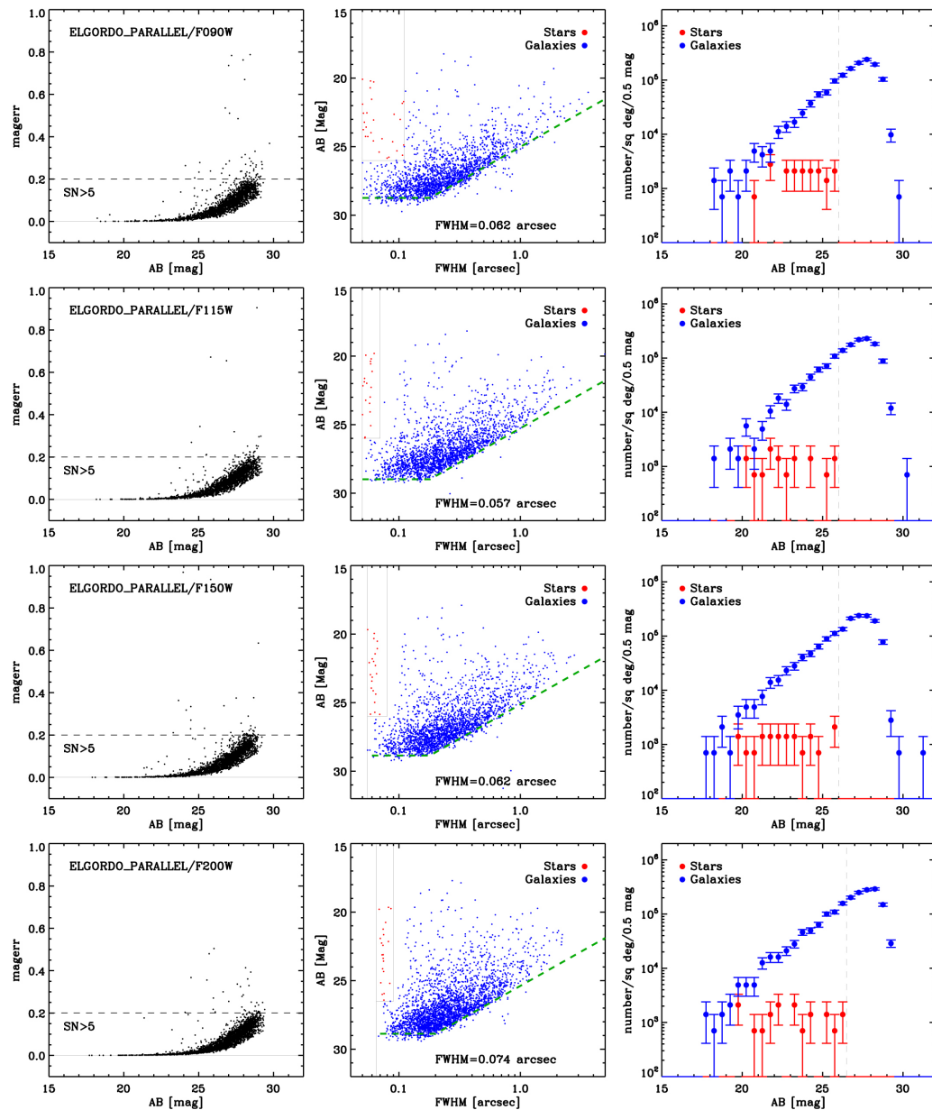
Figure 6. from Rogier A. Windhorst et al 2023 Astron. J. 165 doi:10.3847/1538-3881/aca163 https://dx.doi.org/10.3847/1538-3881/aca163 © 2022. The Author(s). Published by the American Astronomical Society.
