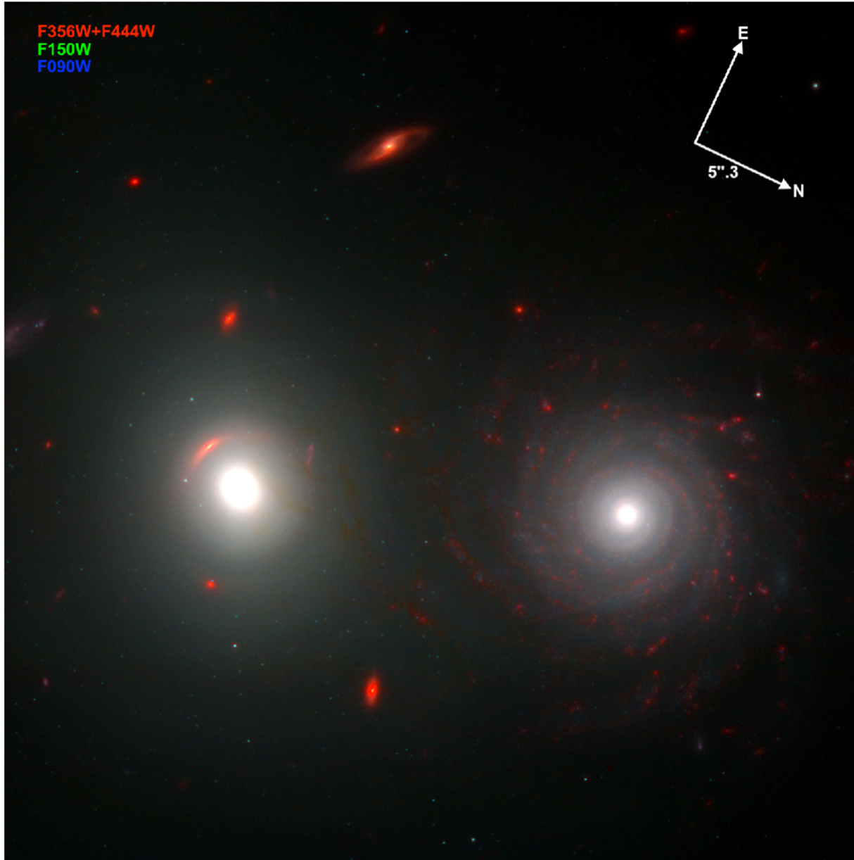
Figure 5. from Rogier A. Windhorst et al 2023 Astron. J. 165 doi:10.3847/1538-3881/aca163 https://dx.doi.org/10.3847/1538-3881/aca163 © 2022. The Author(s). Published by the American Astronomical Society.
