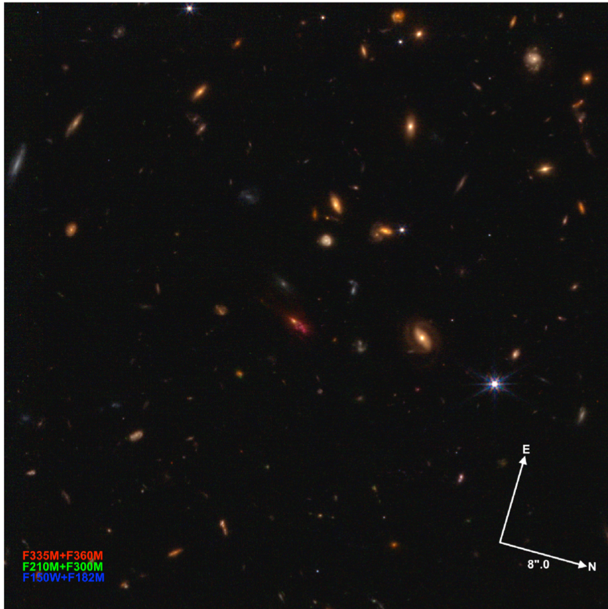
Figure 4. from Rogier A. Windhorst et al 2023 Astron. J. 165 doi:10.3847/1538-3881/aca163 https://dx.doi.org/10.3847/1538-3881/aca163 © 2022. The Author(s). Published by the American Astronomical Society.
