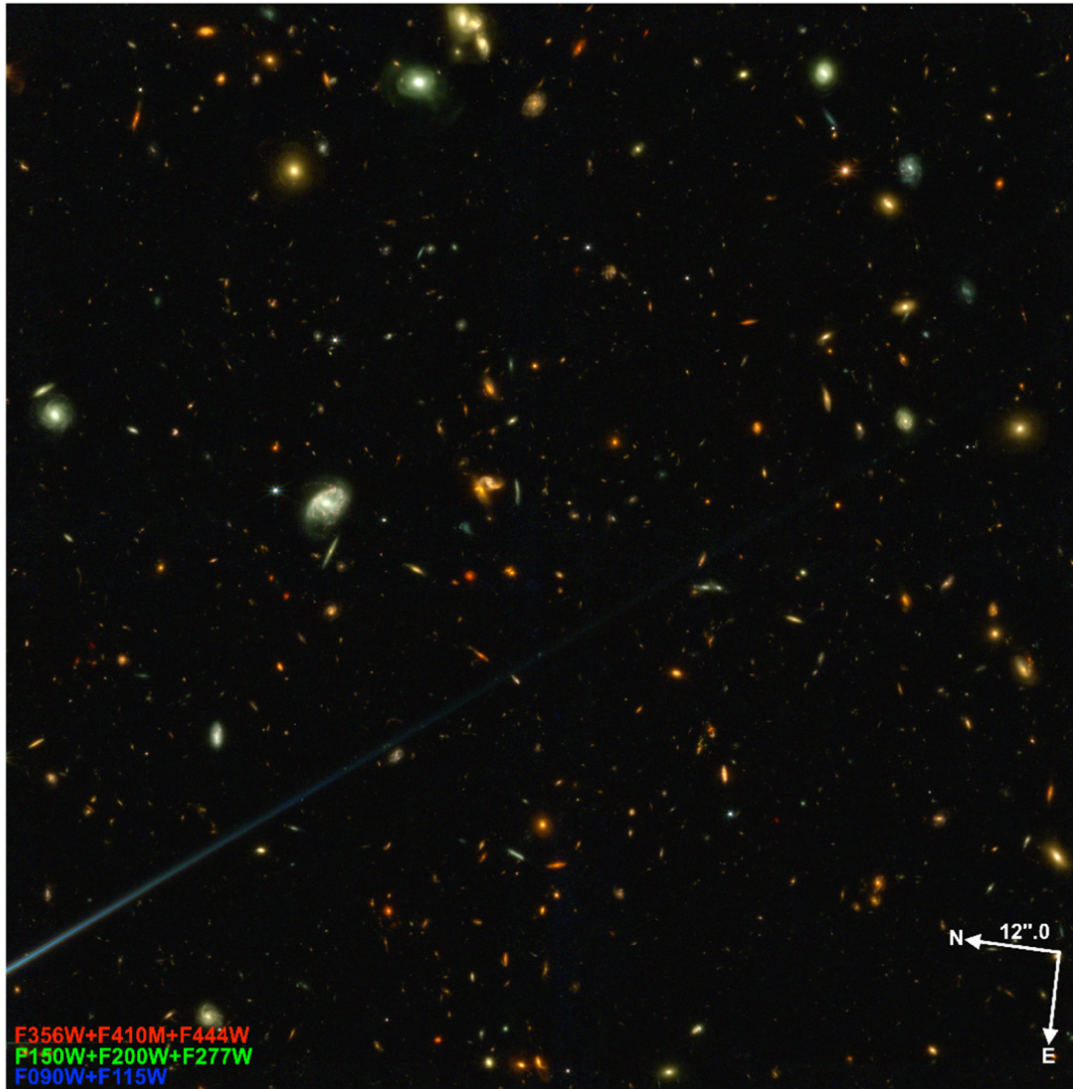
Figure 3. from Rogier A. Windhorst et al 2023 Astron. J. 165 doi:10.3847/1538-3881/aca163 https://dx.doi.org/10.3847/1538-3881/aca163 © 2022. The Author(s). Published by the American Astronomical Society.
