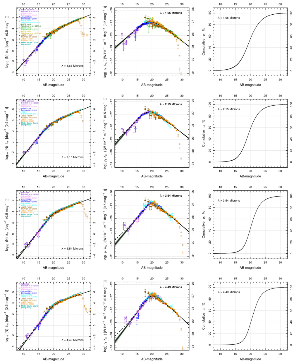
Figure 10. from Rogier A. Windhorst et al 2023 Astron. J. 165 doi:10.3847/1538-3881/aca163 https://dx.doi.org/10.3847/1538-3881/aca163 © 2022. The Author(s). Published by the American Astronomical Society.
