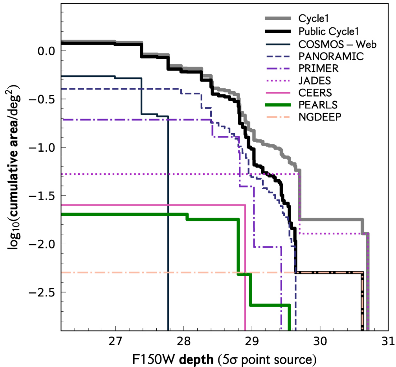
Figure 1. from Rogier A. Windhorst et al 2023 Astron. J. 165 doi:10.3847/1538-3881/aca163 https://dx.doi.org/10.3847/1538-3881/aca163 © 2022. The Author(s). Published by the American Astronomical Society.
