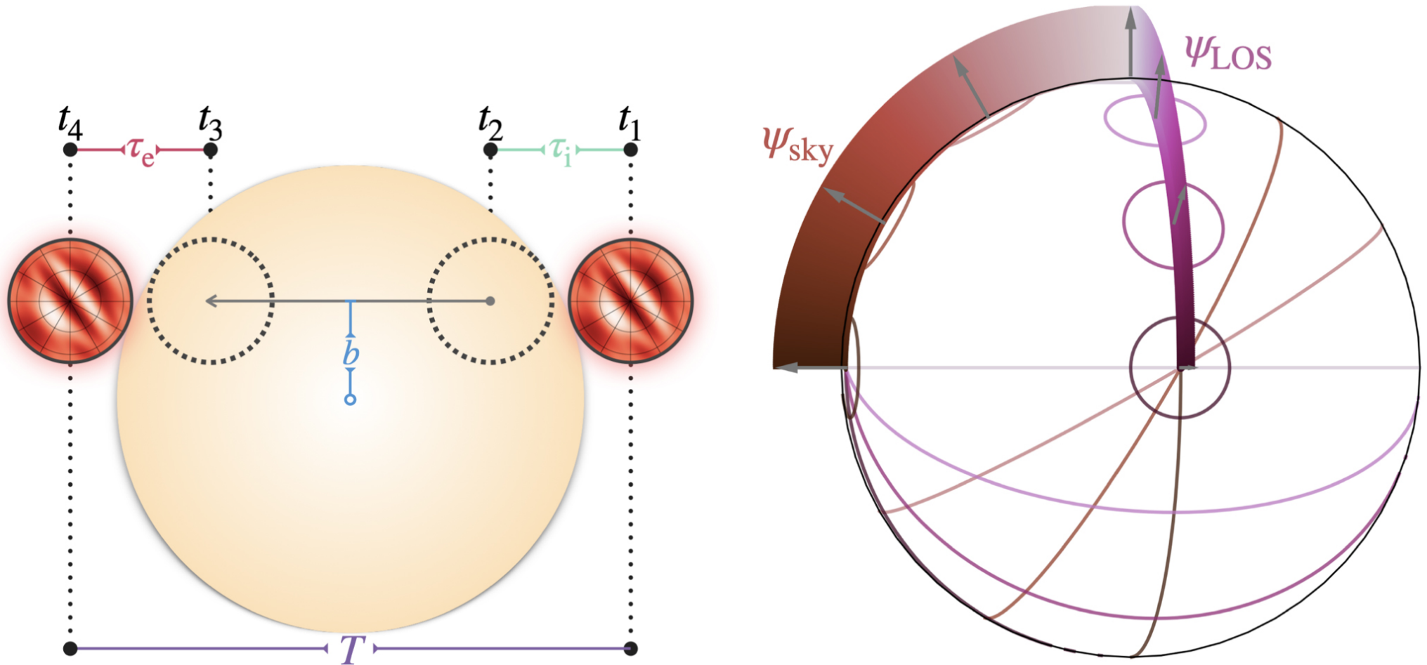
Figure 2. from Arthur D. Adams and Emily Rauscher 2023 Astron. J. 165 doi:10.3847/1538-3881/ac9f46 https://dx.doi.org/10.3847/1538-3881/ac9f46 © 2022. The Author(s). Published by the American Astronomical Society.
